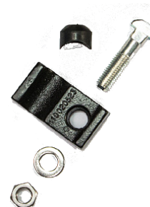
f BRIDE + GOUJON+ ECROU+RONDELLE+ JOINT S4 LAC 5 BUV_1090860
